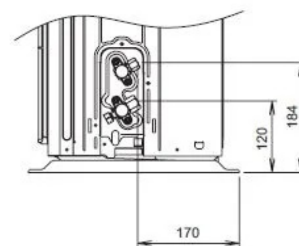
Side view (Valve part)
